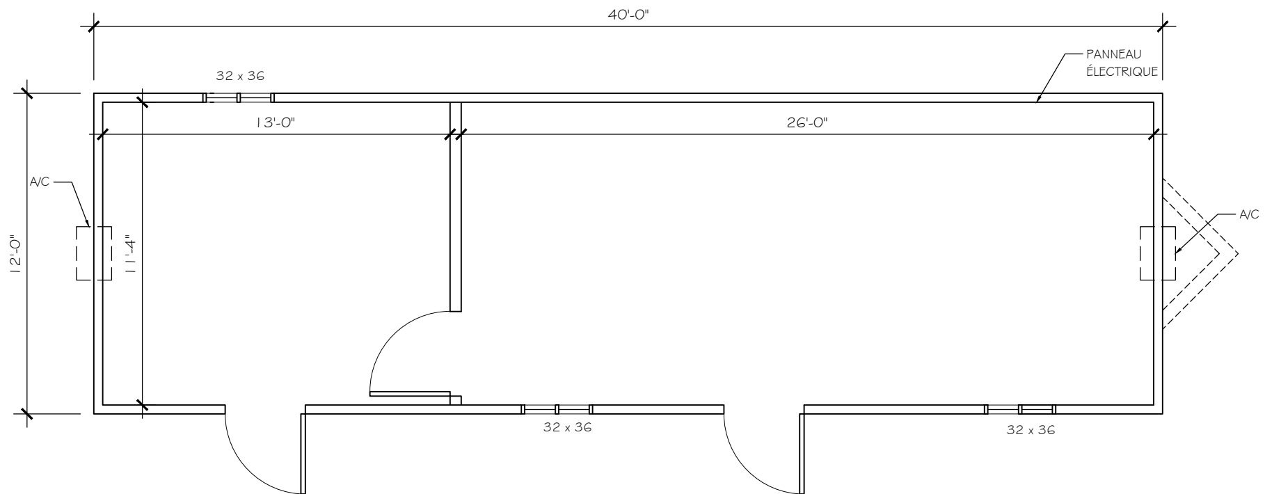
ROULOTTE #05 - 12' X 40'
